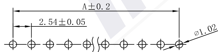
P C B LAYOUT
