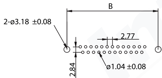
P.B.C BOARD HOLE LAYOUT P.B.C LAYOUT TOLERANCE:±0.05mm
