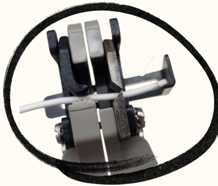
Stripping length stopper
