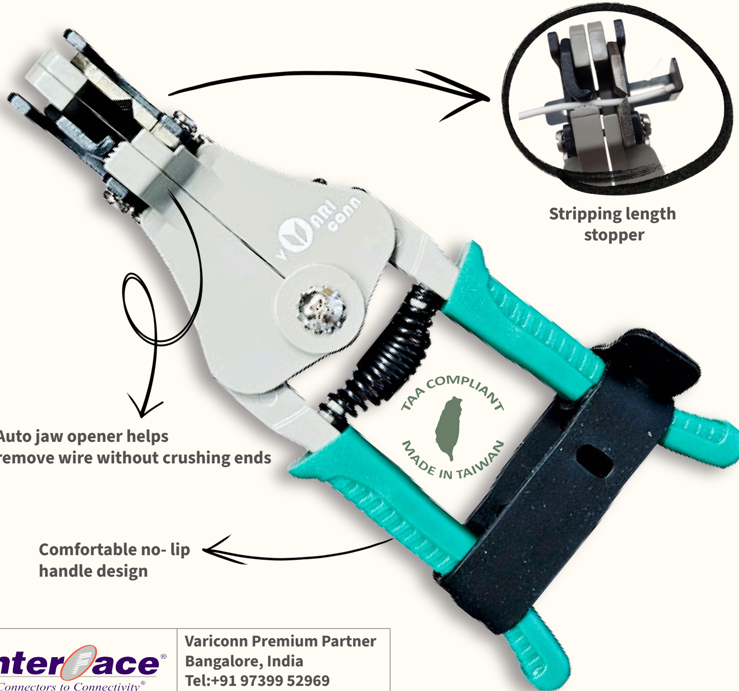
Adjustable stripping length guide
